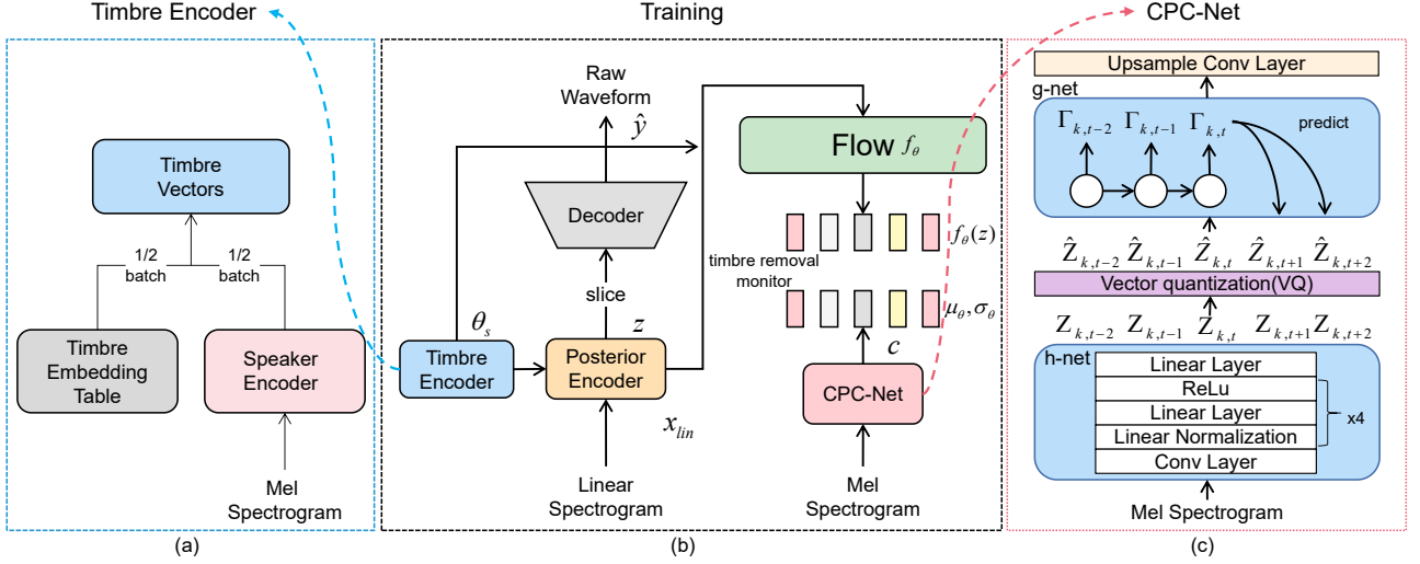
Figure 1: The architecture of FlowCPCVC. (a) Timbre vectors from speaker encoder or timbre embedding table. (b) Overall procedures for training. (c) Architectural components of CPC-Net.
